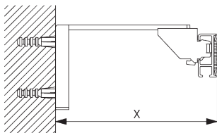
Smart Fix SG 11200 - SG 11205:
