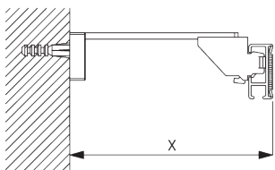
Square Smart Fix SG 11210 - SG 11215:
