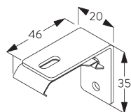
SG 2343 Bracket 46 mm
